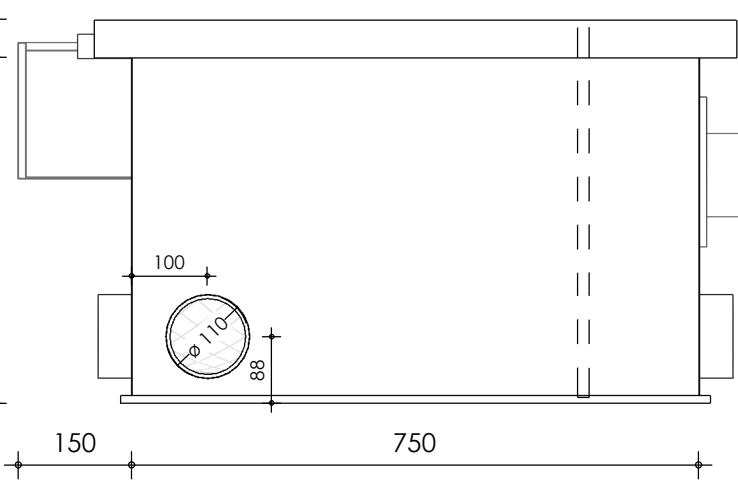
Left-side view
